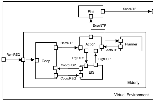
Fig. 2. Refined Virtual Environment for Testing Autominder
