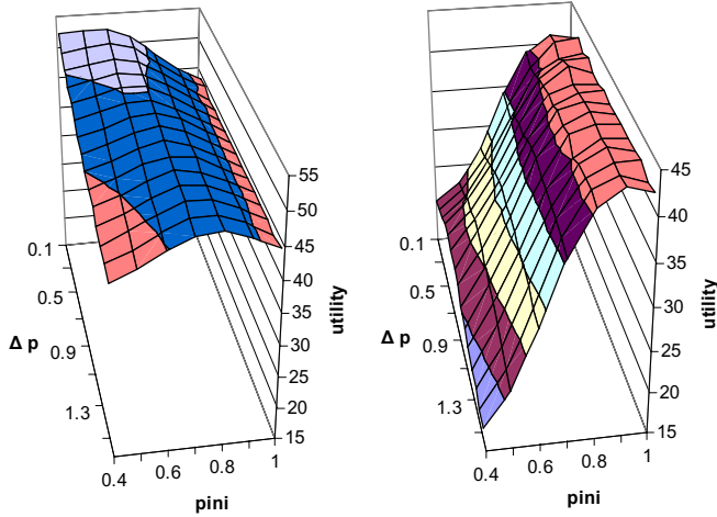
Fig. 4. Utility of the test bidder for quantity maximizing preference \beta = 0.01 (left) and impatient bidding behavior \beta = 1.0 (right) for determination of the optimal bidding strategy under varying price increment \Delta p and initial pricing behavior P^{ini}
