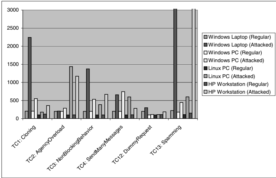
Fig. 2. JADE DoS test results (execution time in msecs)
