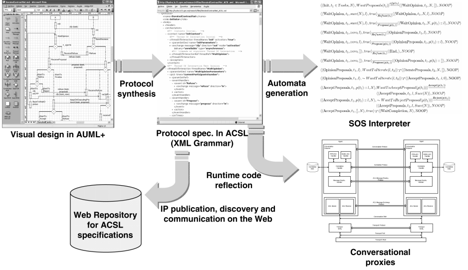
Fig. 1. Tools and artifacts of the DIALOG framework
