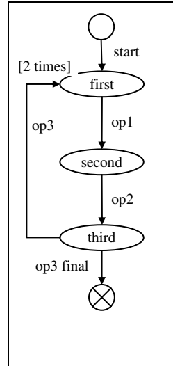
Fig. 5. Simple Jade behavior example: 3 states automaton, with the corresponding finite state automaton diagram on the right
